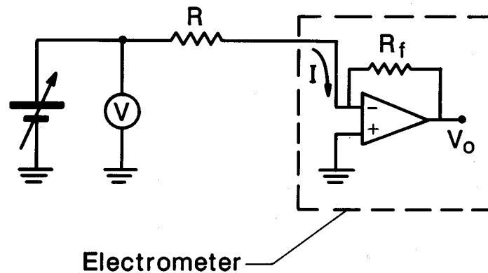
Figure 10 — Schematic View of a Current Injection Circuit for Calibrating Electrometer Used With Wilson Plate
